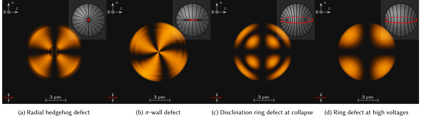
Fig. 4. E12 liquid-crystal microdroplets rendered under cross-polarized light. The droplets are of 9\mu\text{m} in diameter, illuminated by a 590\text{ nm} light. The configuration of the director field (with defects illustrated in red) as well as the orientation of the polarizers are depicted in the top right and bottom left corners of the figures, respectively. The E12 nematic admits an ordinary refractive-index of 1.52 and an extraordinary refractive-index of 1.74 at room temperature and at 590\text{ nm} radiation. The refractive-index of the surrounding isotropic PDMS (polydimethylsiloxane) is 1.43. Due to the rapid change of the optic axis, especially at the center in the radial configurations (a-b), artefacts arise due to accuracy fall-off of the method. Numeric imprecision errors also arise around the edges. For comparison, micrographs of microdroplets with topologies similar to (b) and (d) can be seen in figure 5. See subsection 5.1 for further discussion.
