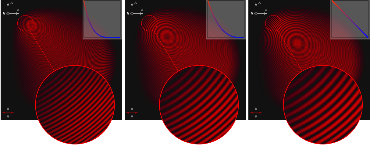
Fig. 7. Fringe patterns that arise as a result of interference as light refracts through a E44 liquid-crystal plate of thickness \tau = 0.80 mm. Viewed under cross-polarizers and 640 nm light. One side of the plate was heated to 368 K while the other remains at 278 K, causing a temperature gradient that gives rise to non-uniform changes in the liquid-crystal's refractive-indices. As a result, the distance between the fringes depends on the heat diffusion. The extraordinary refractive-index of the E44 is modulated from 1.8235 ( T = 278 K) to 1.7035 ( T = 368 K), while the ordinary refractive-index remains fixed at 1.53. The state of the heat diffusion process is illustrated in the upper right corner as a plot: The x -axis corresponds to depth in the plate while the y -axis is temperature. The figures are in chronological order from left to right, such that the figure on the left happens just after the process begins and the figure on the right is once equilibrium is reached. Note that while the heat distribution and incident energy are azimuthally symmetric, the director field is not and therefore the pattern is not radial. The director field is constant and set to about -\frac{1}{2\sqrt{2}}\hat{x} + \frac{1}{2\sqrt{2}}\hat{y} + \frac{\sqrt{3}}{2}\hat{z} . See figure 8 and subsection 5.2 for an overview of the experiment.
