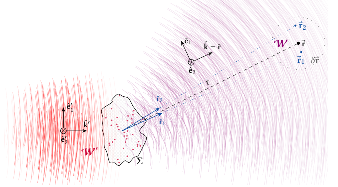
Fig. 3. Diffraction of natural light by an obstacle \Sigma . The obstacle may be any matter or medium or, equivalently, an opening in a conductive screen (i.e. an aperture). An incident field (wavefronts illustrated as red lines), with its coherence properties quantified by \mathcal{W}' , induces electromagnetic excitations in \Sigma (small purple balls), giving rise to diffracted radiation (wavefronts illustrated as purple lines). The solution to the diffraction problem is then \mathcal{W} , which quantifies the diffracted wave ensemble that has propagated to some point \vec{r} . The wavevectors \hat{\mathbf{k}} and the orthonormal bases \hat{\mathbf{e}} are illustrated as well. Note, as the diffracted wave ensemble propagates the wavefronts become more similar, illustrating that light gains coherence on propagation.
