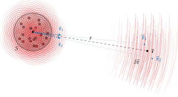
Fig. 2. A spherical natural light source of volume S is centred at the origin o . The source consists of very many elementary radiators (illustrated as red balls) that radiate isotropically (wavefronts illustrated as red curves). This gives rise to the highly chaotic radiation that we call natural light . To quantify the statistical properties of such light that has propagated a distance r to a small region \delta\vec{r} far from the source, we examine the statistical similarity of the wave ensemble at some points \vec{r}_1 and \vec{r}_2 (in directions \hat{r}_1 , \hat{r}_2 from the center of the source) in that region.
