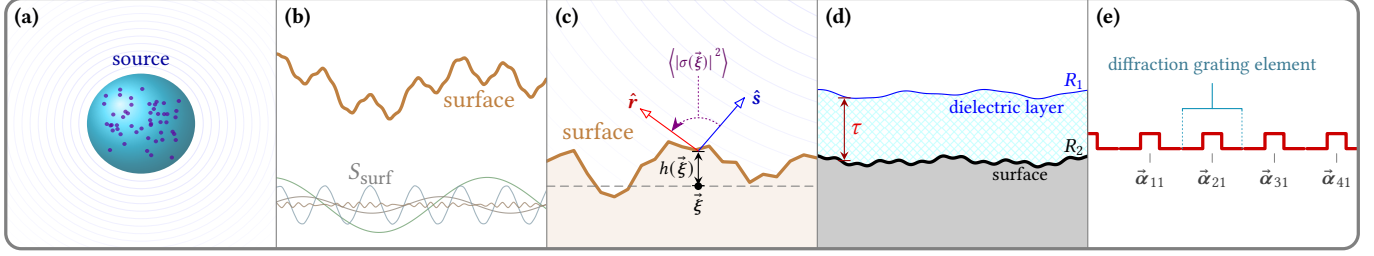
Fig. 6. Examples of light-matter interaction that we discuss in this paper. (a) Sourcing of partially-coherent light: Charges and current in a light source give rise to electromagnetic radiation. The amount of charge together with its spatial correlation fully describe the emitted radiation and its coherence properties. (b) Scatter by a statistical surface: A surface (brown) is decomposed into its spatial frequencies (illustrated in gray). The power of each frequency is given by the power spectral density (PSD) function S_{\text{surf}} , which plays an important role in describing the scattered radiation. (c) Scatter by explicitly-defined microgeometry: A surface patch is described by the (explicit) height perturbations h(\vec{\xi}) , where \vec{\xi} is a point on the surface plane (gray dashed line). As always: \hat{s} , \hat{r} are the incident and exitant directions and \langle |\sigma(\vec{\xi})|^2 \rangle is the (ensemble-averaged) reflectivity (i.e. scattered intensity). (d) Layered structure: A dielectric layer over a substrate, where the surface of each is described statistically via the stationary autocorrelation functions R_1 and R_2 , respectively. The surfaces are assumed to be statistically independent. (e) Diffraction grating: A two-dimensional grid of small and identical, but otherwise arbitrary, optical elements produces a diffraction grating. The elements are regularly spaced and the position of the center of each element is denoted \vec{\alpha}_{pq} .
