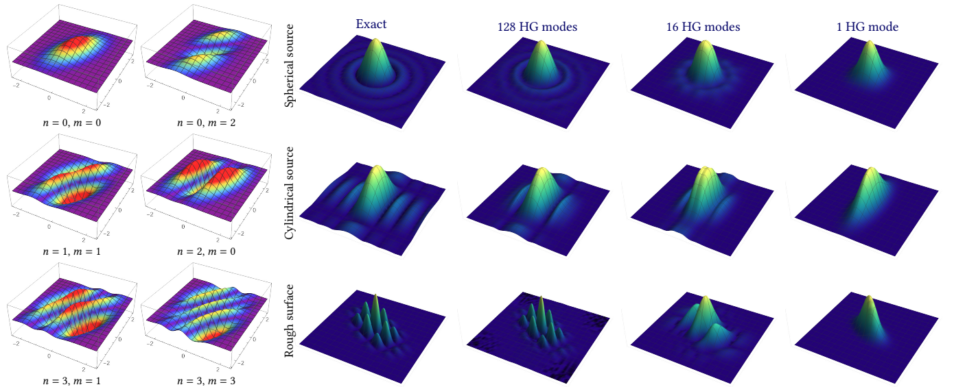
Fig. 4. (left) A few even-ordered anisotropic Hermite-Gauss transverse modes. The shape matrix \Theta of the presented modes encodes a rotation and an anisotropic scale, i.e. \Theta^{-1} = R S (R S)^T , where R is a rotation matrix of \frac{\pi}{7} radians (around \hat{z} ) and S is a diagonal scale matrix with a scale of 2 in \hat{x} and 1 in \hat{y}, \hat{z} . (right) The HG modes form a functional basis that is able to express a wide variety of CSD functions using a limited number of modes. Observe that as the shape matrix encodes the coherence shape and area, even with a single mode we can capture some of the important characteristics of the CSD.
