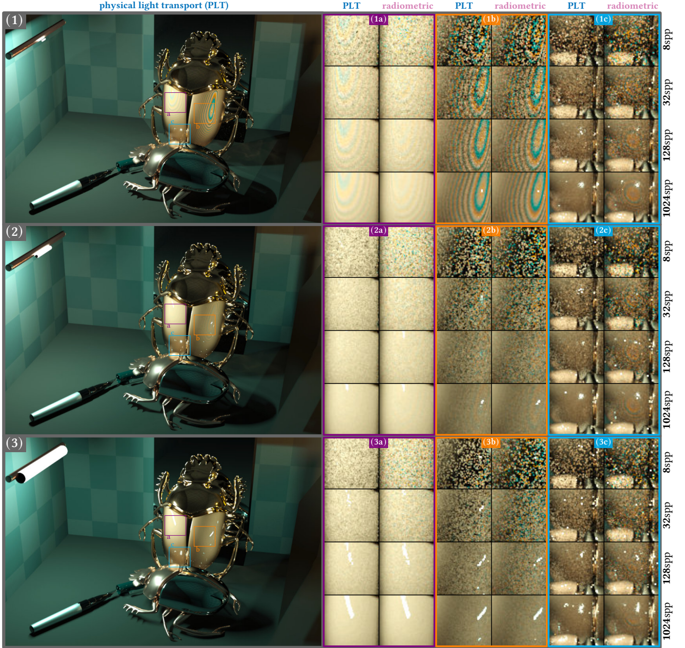
Fig. 8. (left) A large golden scarab with polished body and unpolished, rough wings, that are coated with a moderately thick dielectric, is illuminated by a short-spectrum light source of varying size. A smaller copper scarab with rough body and (uncoated) polished wings is placed at the bottom. A rectangular mirror, on the right, reflects light from the source back towards the golden scarab. The mirror and the polished small scarab's wings act as Dirac delta perfect reflectors (see Section 5). Hence, light incident upon the golden scarab after reflection off the mirror is more coherent than light that arrives directly from the source: the right wing showcases more pronounced interference patterns than the left. Rendered with 8192spp. (right) We compare our coherence-aware physical light transport (PLT) with radiometric light transport (RLT) where the golden scarab's wings are rendered the method by Belcour and Barla [2017]. Each of the insets is a close-up on an area outlined in the full image, rendered with increasing samples-per-pixel. RLT mimics spatial coherence by superpositioning many plane waves sourced from different points on the source and insets (a,b) show decent agreement between the produced patterns. However, to avoid aliasing many such samples are needed: observe the colourful noise artefacts in the RLT insets, which mostly disappear only with 1024spp and do not exist at all with PLT. The required sample count becomes particularly untenable with indirect weakly-coherent illumination, which is highlighted in insets (c): this area is illuminated indirectly by light diffused by the rough body of the small scarab. The close proximity of the small scarab and its body's rough surface mean that this light is very weakly-coherent (note the size of the diffused highlight on the rough body and invoke the VCZ theorem), an effect correctly captured by our method but not RLT: observe the erroneous diffraction patterns that appear. Both methods admit similar rendering times with identical sample count. High-resolution renderings are available in our supplemental material.
