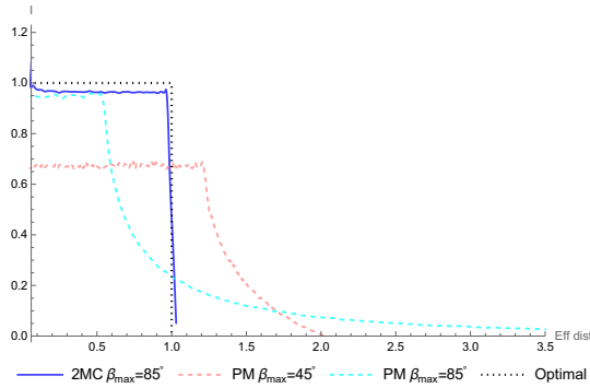
Fig. 5. Intensity distribution for concentration along one dimension on a flat target, L = 20f , \epsilon = 0.01 .
