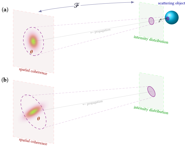
Fig. 6. Illustration of light that is scattered of the surface of an object. The intensity distribution on the transverse plane of the scattered beam is illustrated on the green plane on the right. This intensity distribution is related to the spatial coherence function of the light on the transverse plane after propagation (red plane on the left) via a Fourier transform. (a) If the material scatters isotropically and the intensity distribution is isotropic, then the spatial coherence must be isotropic as well. (b) On the other hand, anisotropy in the scattering characteristics might induce deformations in the beam. Then, the spatial coherence after propagation undergoes a transformation that is the inverse of the intensity distribution's transformation. This transformation of the spatial coherence on the transverse plane is in fact the leading principal minor of the shape matrix \Theta .
