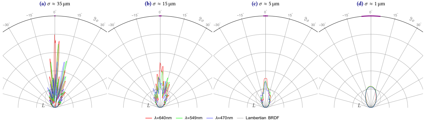
Fig. 5. The wave BSDF (wBSDF): Plots of the radiance L = L_x + L_y scattered by a scratched metal surface. Incident light with unit irradiance impinges upon the surface at normal incidence. Three different representative wavelengths are used as well as light of different spatial coherence area: (a) comparable to sunlight; (b) moderately coherent; (c) weakly coherent; and (d) highly diffused. Also plotted are Lambertian BRDF lobes, viz. \frac{1}{\pi} \cos \vartheta_o , where \vartheta_o is the scattering angle, in gray, for comparison. The standard deviation \sigma of the characteristic length of spatial coherence on the transverse plane is listed. Incoherence is equivalent to an angular blurring of the wave BSDF (convolution with the inverse coherence Gaussian), and we illustrate the angular magnitude of the blur using the purple lines at the top of the plots. An important distinction between the classical BSDF and our wBSDF is that, due to constructive wave interference, the scattered power ratio \partial\Phi^{(o)} / \partial\Phi^{(i)} may now surpass unity (assuming \Omega^{(i)} = \Omega^{(o)} , where \Omega is the solid angle into which a beam propagate, and assuming no re-emission effects, like fluorescence). Nevertheless, energy must be conserved over the entire scattering codomain (the unit sphere or hemisphere).
