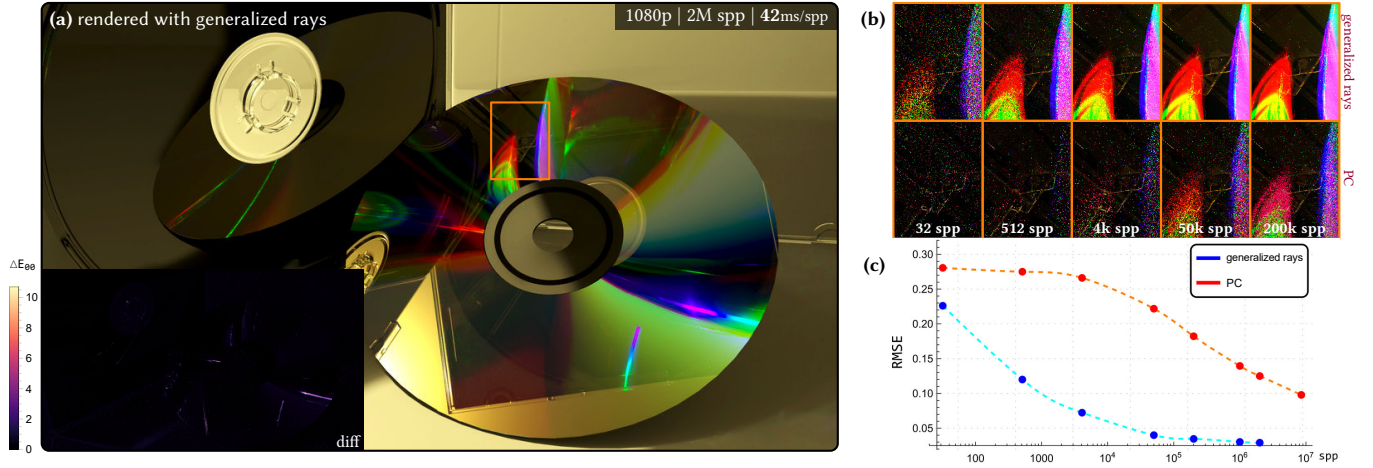
Fig. 7. Partially-coherent sampling. (a) A scene contains a compact disk (CD) that rests next an open CD case, upon which another closed CD case is placed. A ceiling-mounted light source illuminates the scene. While simple, the scene admits interesting light transport. (b) We emulate partially-coherent (PC) sampling of BSDFs, in an identical manner to the state-of-the-art (PLT), which manifests the sampling problem: the diffraction lobes are very sharp lobes that are difficult to sample when doing backward path tracing (and the coherence properties of light are unknown) using existing tools. The close ups show the area marked in orange rendered at various sample counts. Note the sharp difference in noise between PC sampling and our proposed light transport formalism with generalized rays. (c) Plot of noise as function of sample count, quantifying the drastic improvement in sampling performance: sampling using generalized rays reduces sample count by a factor of about 4000 for similar-quality rendering. (a, inset) A difference image between the two sampling strategies. With the exception of the very high-frequency diffraction effects, the differences are minor, and are due to the PC rendering never converging.
