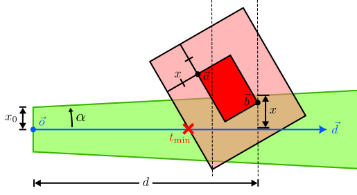
Figure 12: Elliptical cone–ABB intersection for 8-wide BVH is done via a conservative ray–ABB intersection with the ABB enlarged by the cone’s maximal cross section size x . Dashed lines indicate accurate cone–ABB intersection range, while the nearest point (red cross) computed with this test serves a conservative approximation.
