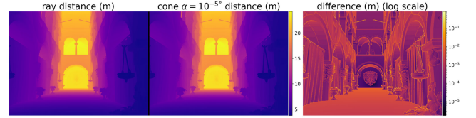
Figure 4: We test the numerical stability and robustness of cone–triangle intersection by visualizing the distance to closest intersection point for tiny cones with \alpha = 10^{-5} compared with rays. Cones always intersect the surface at a distance that is equal or less compared with a corresponding ray, though the difference is very small except at object silhouettes.
