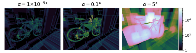
Figure 6: Heatmaps (log scale) of revisited triangle count in a K-d tree traversal. The count of revisited triangles increases with cone angle similar to the count of intersected triangles. Revisited triangles constitute a considerable wasted effort in K-d tree traversal.
