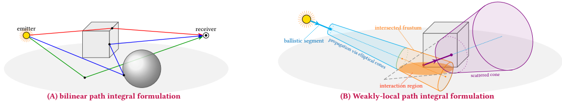
Figure 2: Path integrals for wave optics. We develop two generalizations of the classical light transport path integral [Vea97]—capable of reproducing a wide range of wave effects. (A) The bilinear path integral, Subsection 3.1 (implicitly employed by common methods that use phase-carrying rays, like those that rely on UTD-based diffractions) accounts for the interference between all pairs of paths. Bilinearity frustrates local path sampling: assume that a path was sampled; afterwards, another path might be sampled that destructively interferes with the former path, resulting in overall negligible contribution, even with good local path sampling. (B) The weakly-local path integral, Subsection 3.2 , formalizes region-to-region transport. In-place of rays, we employ elliptical cones for transport, and formulate the aggregated interaction of light with all materials that fall within a region (illustrated in orange). This requires more sophisticated machinery—tracing of elliptical cones and aggregated wave-optical interactions—but allows crucial local path sampling. Ballistic segments are illustrated using thick lines, and an elliptical conic frustum within which intersected geometry is found in orange (see Subsection 4.2 ).
